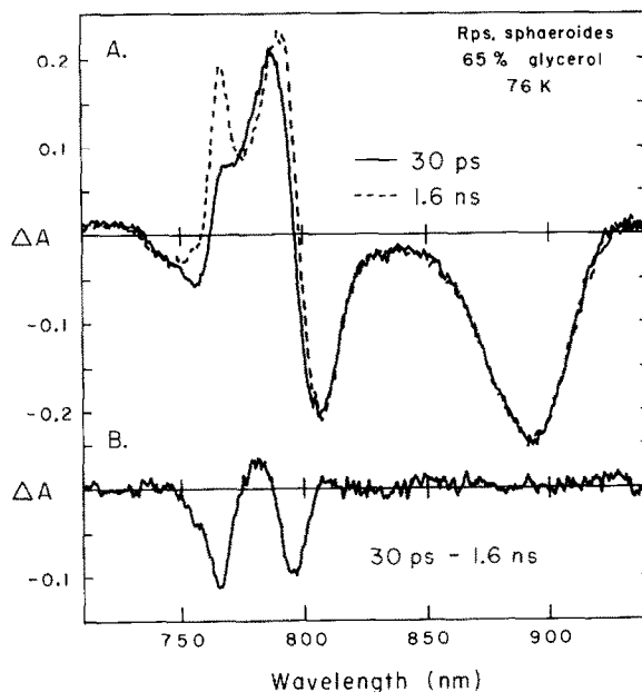
Fig.1. (A) Near-infrared absorption changes at 76 K for Rps. sphaeroides reaction centers in 65% glycerol at 30 ps (—) and 1.6 ns (---) with respect to a 30-ps 600-nm flash. Each spectrum was acquired in two 150-nm slices, that agreed within experimental error in the regions of overlap; each spectrum represents the average of spectra acquired using 300 excitation flashes. (B) Difference between the 30-ps and 1.6-ns spectra in (A).
